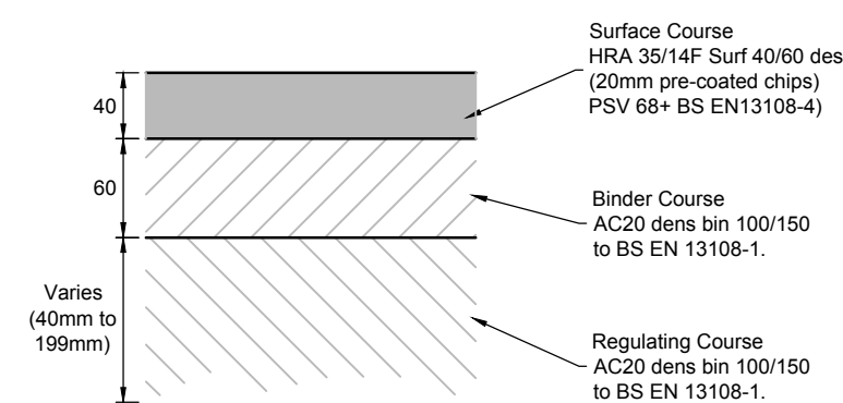
TYPICAL CARRIAGEWAY OVERLAY ON EXISTING CONSTRUCTION WHERE OVERLAY DEPTH IS 40mm to 199mm 1:5
