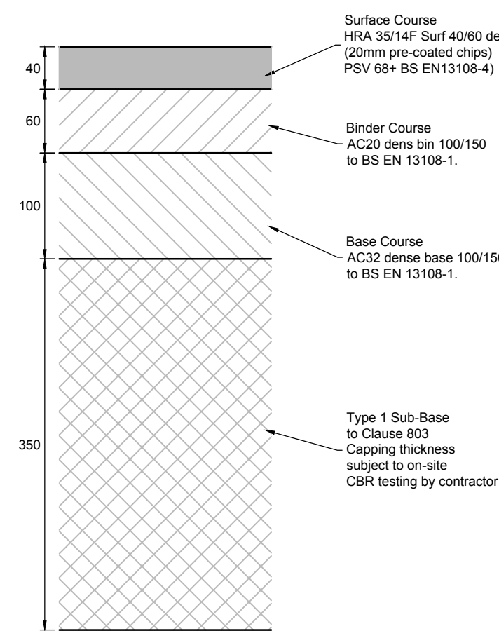
TYPICAL NEW CARRIAGEWAY CONSTRUCTION 1:5
