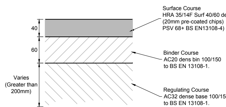
TYPICAL CARRIAGEWAY OVERLAY ON EXISTING CONSTRUCTION WHERE OVERLAY DEPTH IS 200mm or GREATER 1:5
