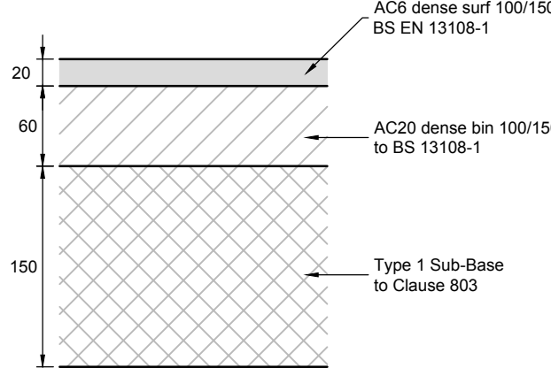
TYPICAL FOOTWAY CONSTRUCTION DETAIL 1:5
